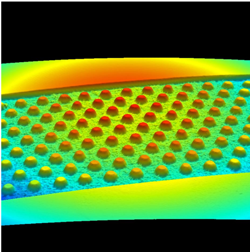
3D measurement of a pillar texture on one of the demonstrator balls.
