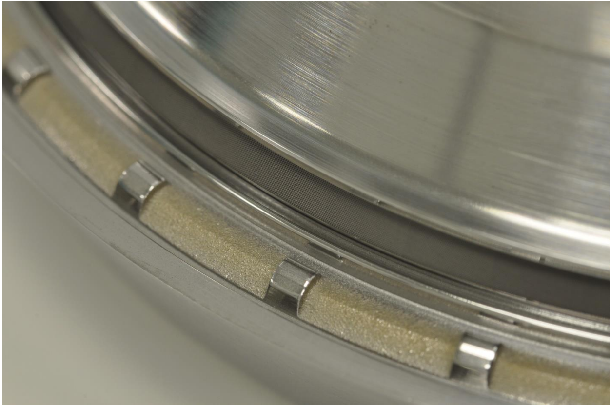
Photograph of a textured mold insert, where a pillar texture was applied to a conical ring around the circumference.
