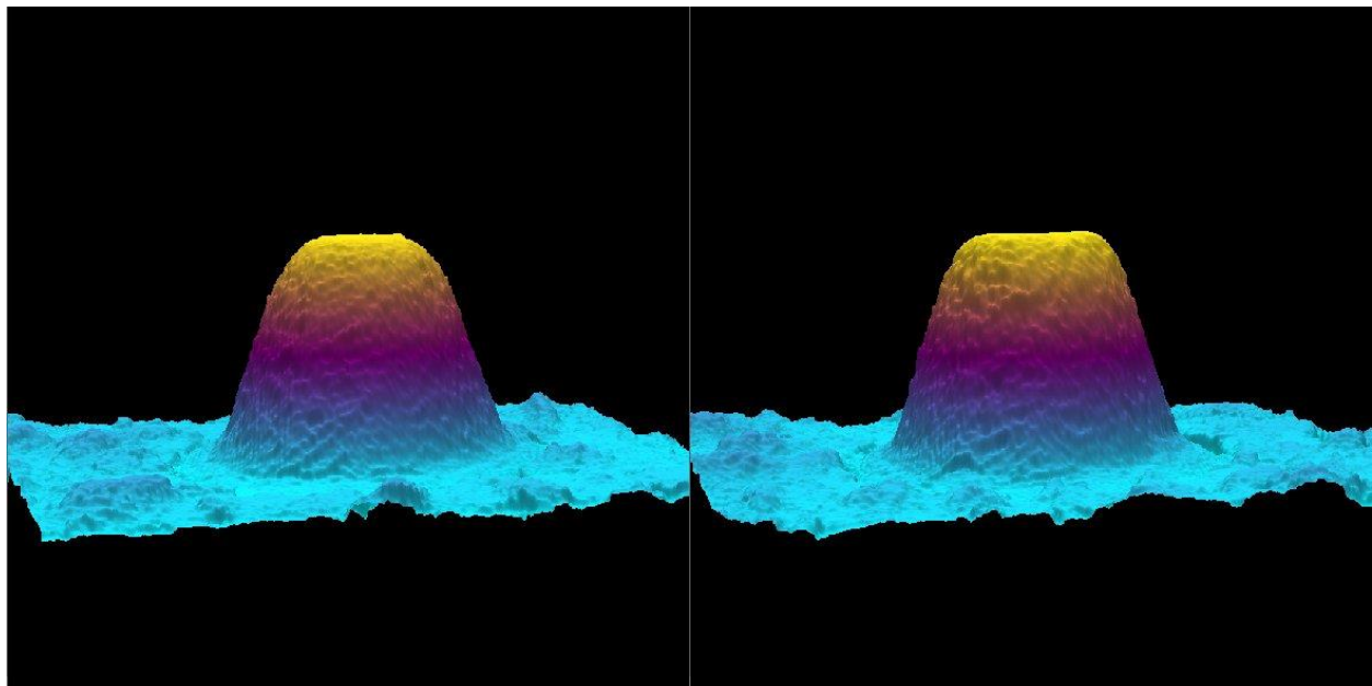
Two images of about 40 \mu\text{m} diameter pillars made with the exact same process (2 m/s scan speed), executed with a standard / 308 kHz pixel clock (left) and using the fast pixel mode (right).
