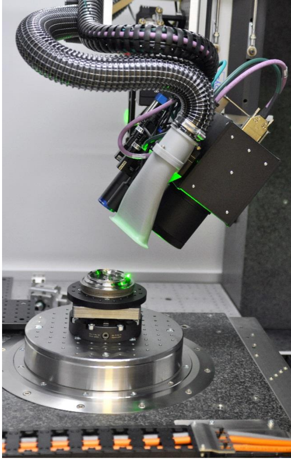
Lightmotif's 5-axis machine during machining of the texture on a mold insert.
